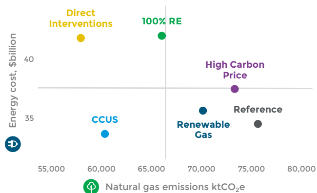
Total energy costs and emissions across pathways
